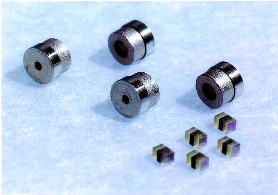
Component of isolator (Faraday rotator is sandwiched with polarization glass)
