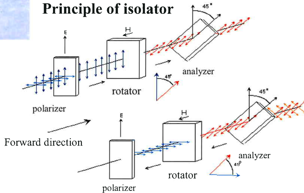
Component of isolator (Faraday rotator is sandwiched with polarization glass)
